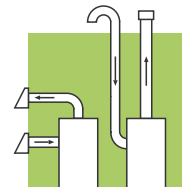
Direct Venting*
