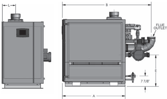
SINGLE HEAT EXCHANGER MODELS Rough In Dimensions (Single)
